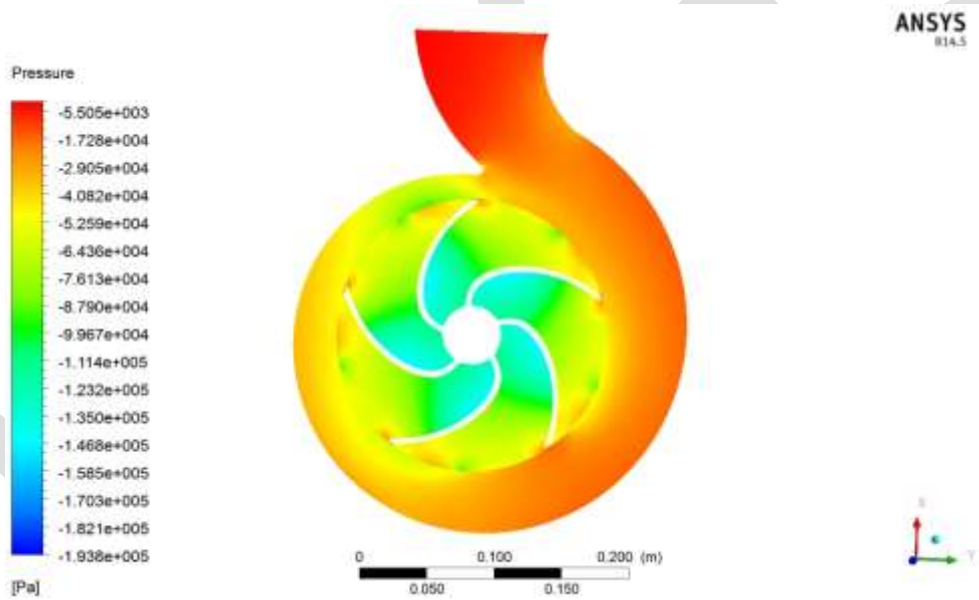
Fig.16: Static pressure distribution for selected PAT model on impeller mid plane at Q = 0.025\text{m}^3/\text{s}
