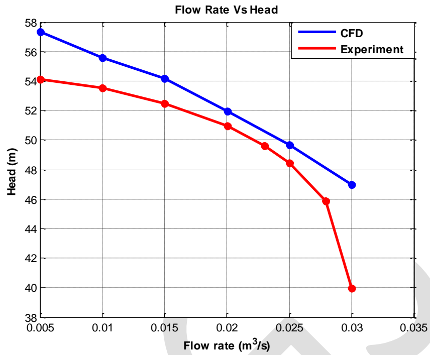
Fig.13: Pump head vs. flow rate characteristics curve of selected pump model at N=2960 RPM
