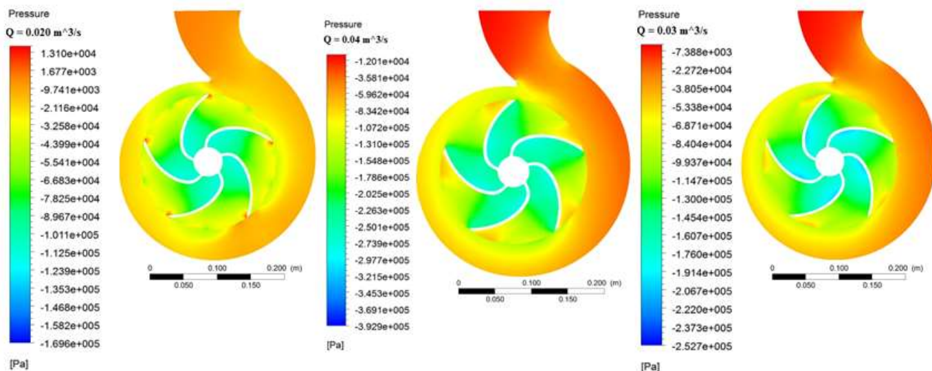
Fig.17: 2D Contour plot colored by static pressure distribution for selected PAT model at different flow rates
