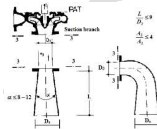
Fig.4: Typical draft tube design and main dimensions (according to Lein) [6].
