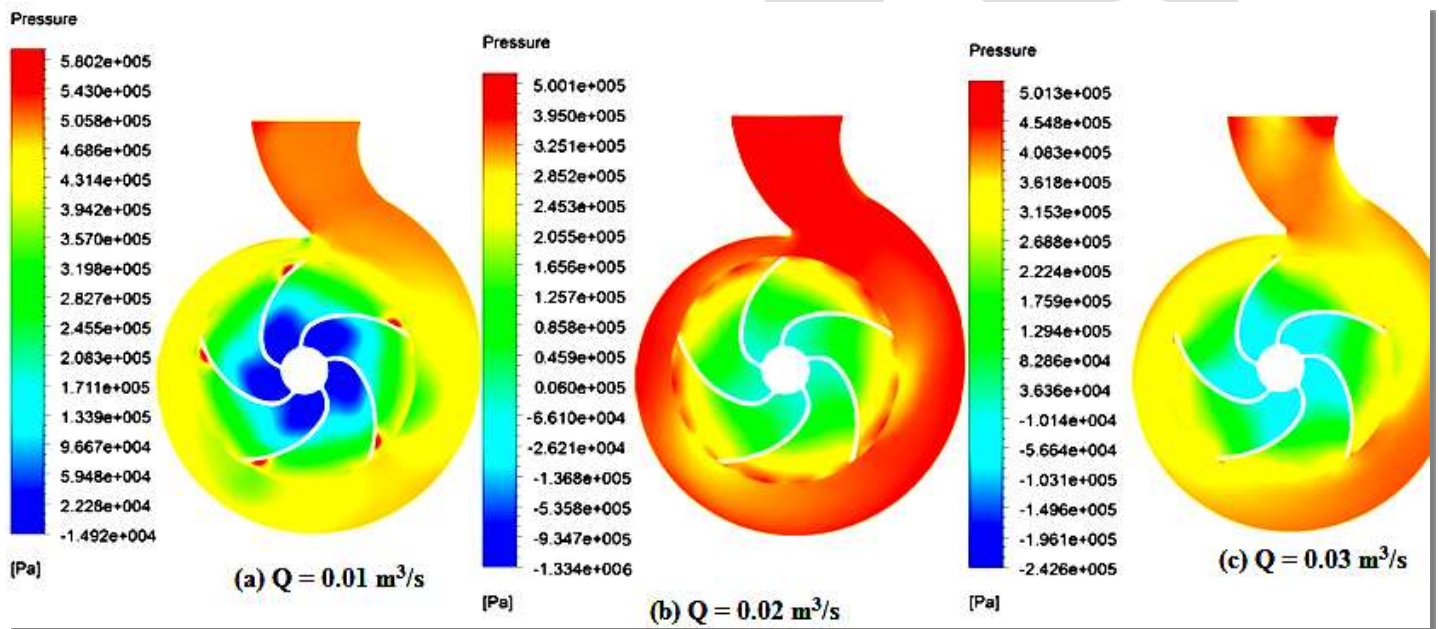
Fig.12: Mid plane static pressure distribution for selected centrifugal pump model at different flow rate.
