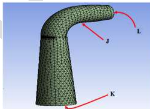
Fig.7: Meshed draft tube fluid domain with PAT boundary names.
