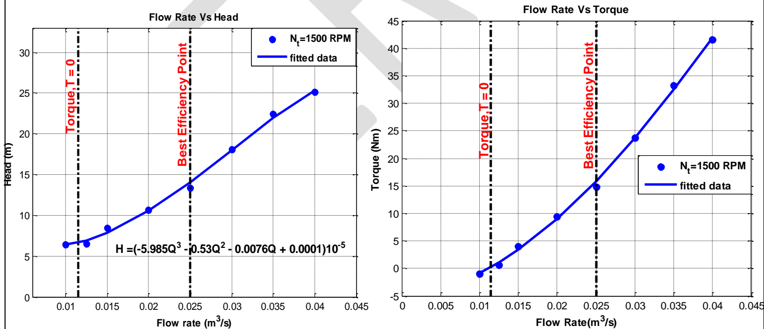
Fig.18: Predicted performance characteristics curves for selected PAT model
