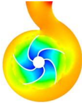
Fig.11: Mid plane static pressure distribution for selected centrifugal pump model at different flow rates.
