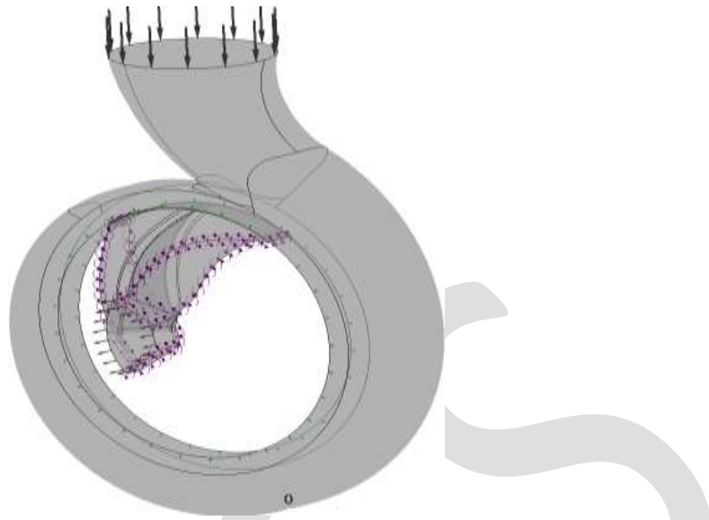
Fig. 9: PAT model with boundary conditions.
