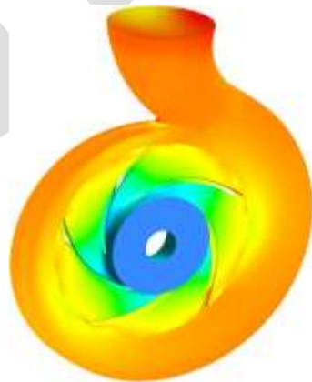
Fig.10: 3D Static pressure distribution for selected centrifugal pump model at Q = 0.025\text{m}^3/\text{s} .
