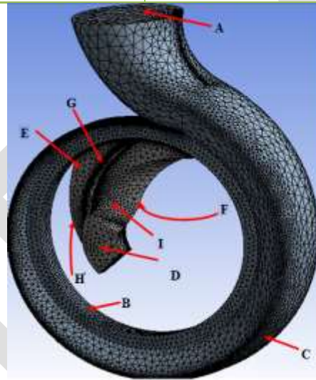
Fig.6: Meshed volute and impeller fluid domains with PAT boundary names.
