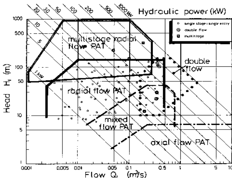
Fig.1: General range of application of different PAT types [6].
