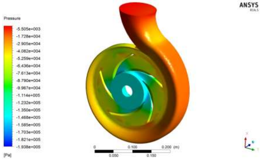
Fig.15: 3D Static pressure distribution for selected PAT model at Q = 0.025\text{m}^3/\text{s}
